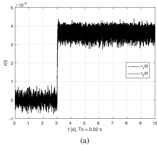
Fig. 2. Responses of the fault residual filter (Theorem 2): the first sector column fault (a), the second sector column fault (b).
