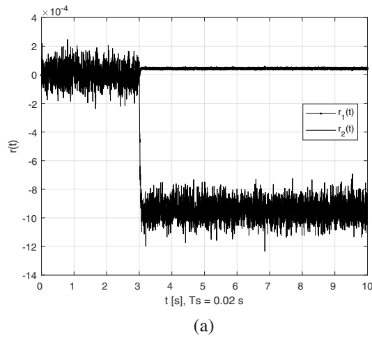
Fig. 1. Responses of the fault residual filter (Theorem 1): the first sector column fault (a), the second sector column fault (b).
