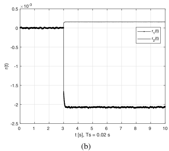
Fig. 3. Responses of the fault residual filter (Theorem 3): the first sector column fault (a), the second sector column fault (b).
