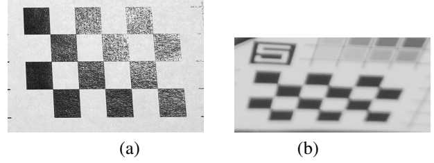
Fig. 6. Examples of undetectable checkerboards due highly reflective paint (a), out of focus caused by an excessively sharp shooting angle (b).
