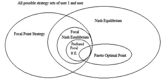
Fig. 1. Relation between various strategies.
