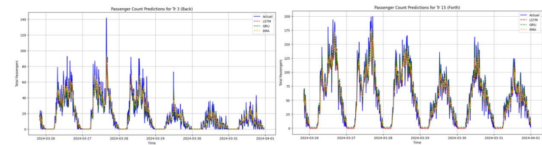
Figure 2. Comparison of LSTM, GRU predictions for Trolleybus 3/Trolleybus 15 (including baseline)
