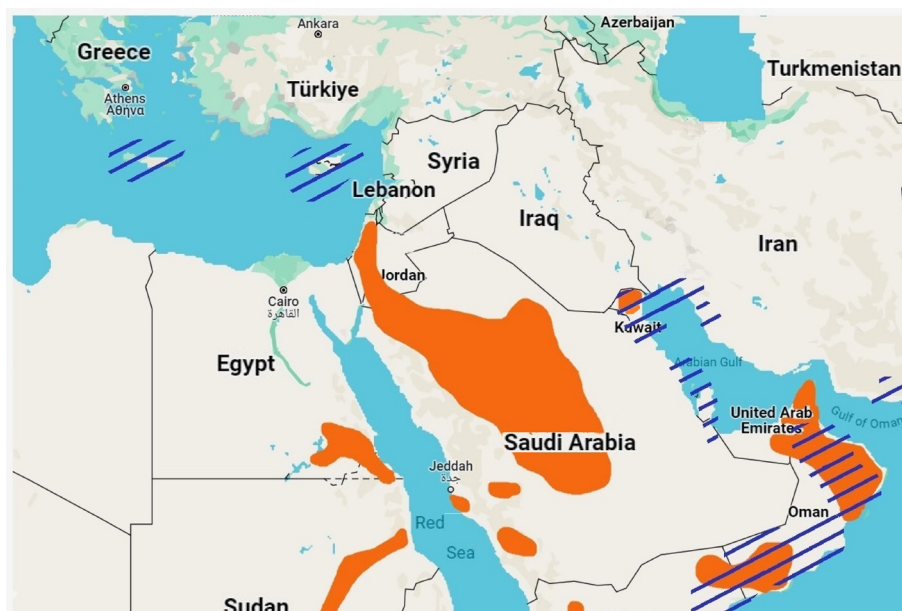
Fig. 1. The distribution of lappet-faced vulture (Orange) and Amur falcon (Blue shade) within the Middle East area. The distribution map was developed based on accumulative data from different dates in the literature.
