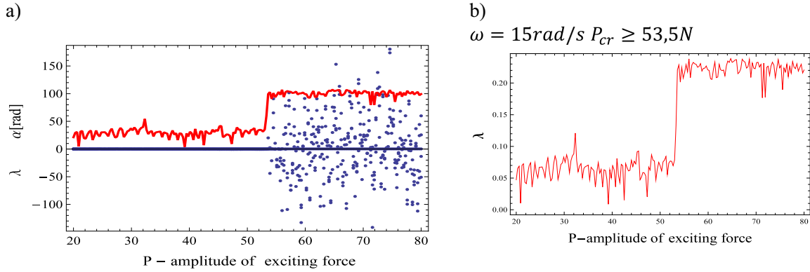
Figure 19. Bifurcation diagram (a) and variation function of max. Lyapunov exponent (b) for the system described by equation (18) \left( L = 0.5 \text{ m}, m = 1 \text{ kg}, k = \frac{100 \text{ N}}{\text{m}}, k_1 = \frac{1,000 \text{ N}}{\text{m}^3}, \omega = 15 \text{ rad/s} \right) .
