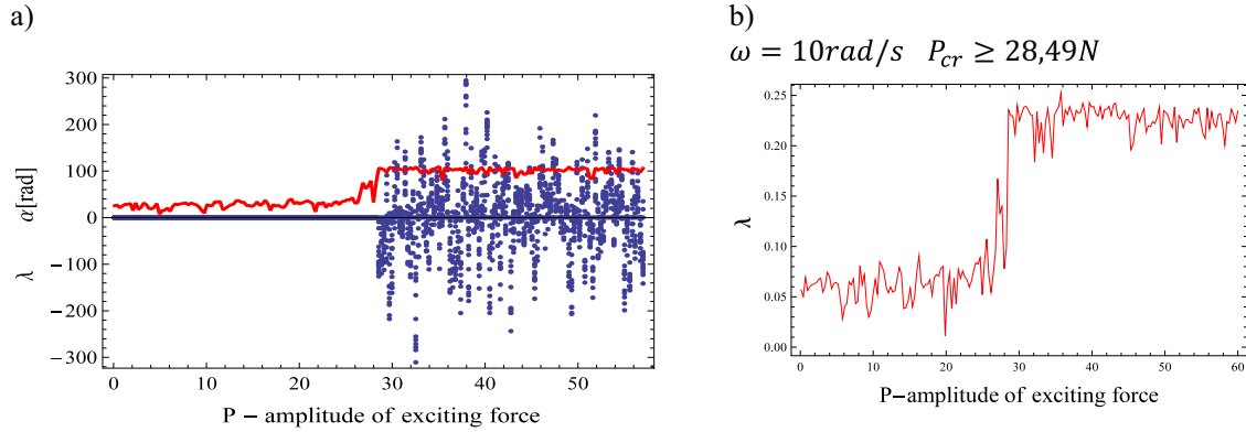
Figure 18. Bifurcation diagram (a) and variation function of max. Lyapunov exponent (b) for the system described by equation (18) \left( L = 0.5 \text{ m}, m = 1 \text{ kg}, k = \frac{100 \text{ N}}{\text{m}}, k_1 = \frac{1,000 \text{ N}}{\text{m}^3}, \omega = 10 \text{ rad/s} \right) .
