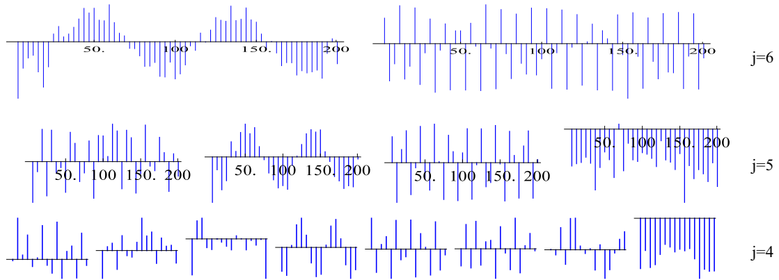
Figure 14. Selected resolution levels j of multiwavelet packet analysis coefficients for nonchaotic signal F = 6.5 of the Duffing oscillator described by equation (17) using packets of Legendre's multiwavelets k3_2.
