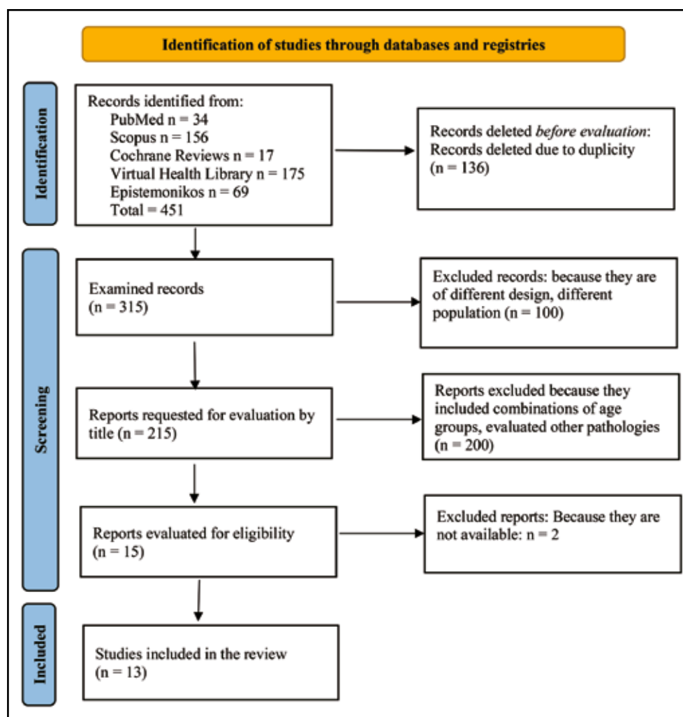
Figure 1. PRISMA flowchart.
