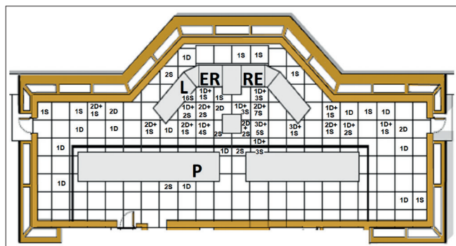
Fig. A.2. Static and Dynamic positions during observation 2 on oil tanker 1
