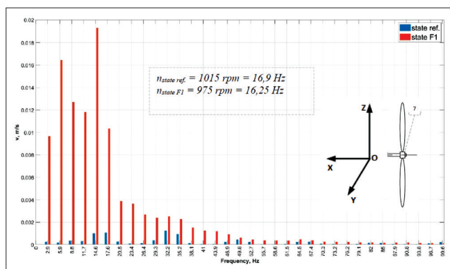
Fig. 12. Vibration velocity spectrum recorded in the OZ direction
