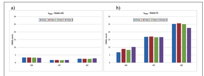
Fig. 9. Summary of the resulting values for each measurement point in: a) state ref., b) state F1
