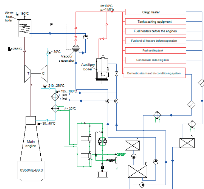
Fig. 5. Schematic diagram of the system for deep heat recovery of high-potential secondary energy resources of the tanker power plant main engine with deadweight of 45,500 tons
