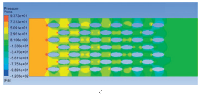
Fig. 2. Results of comparative modelling of flow around profiled pipe bundles: a) bundle of smooth elliptical pipes; b) bundle of pipes with a single notch; c) bundle of pipes with two notches
