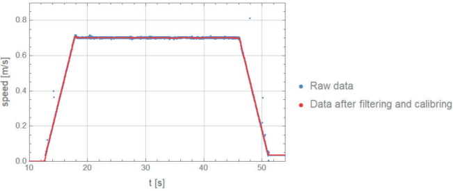
Fig. 3. Smoothing of the speed signal: raw data (blue), after filtering (red) (filtering is needed to retrieve the dynamic model)
