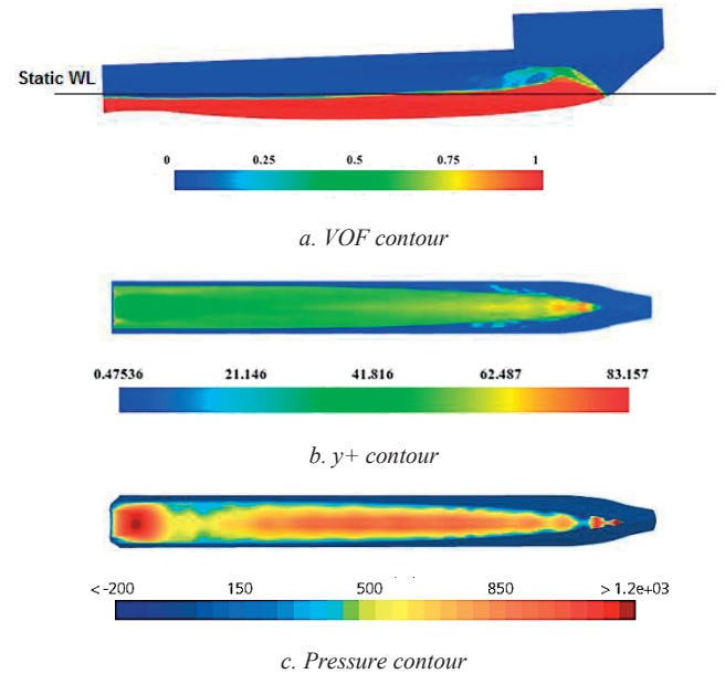
Fig. 4. Detailed features of the AUT-SEM00 model in calm water at a speed of 3.78 m/s
