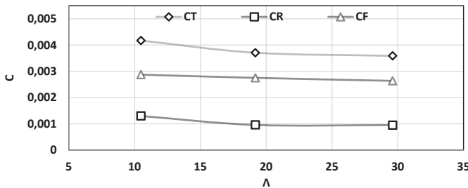
Fig 8. CT, CR, CF versus aspect ratio
