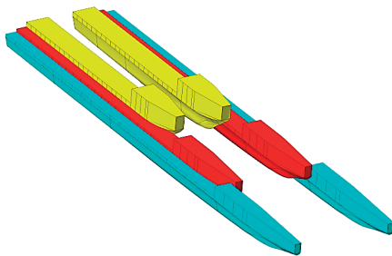
Fig 5. Perspective view of AUT-SEM00 (yellow), AUT-SEM01 (red) and AUT-SEM02 (green)
