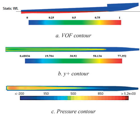
Fig 6. Results for the (a-c) AUT-SEM01 and (d-f) AUT-SEM02 models in calm water at a speed of 3.78 m/s
