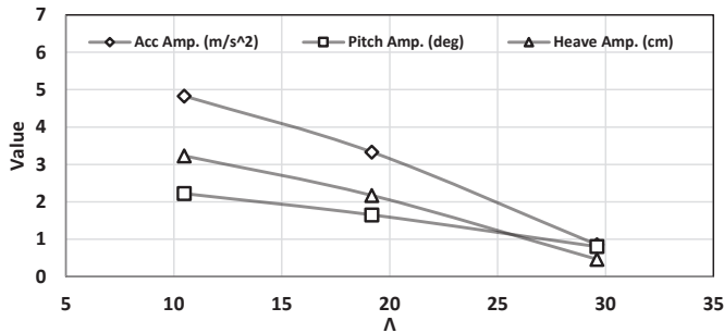
Fig. 11. Effect of aspect ratio on the performance of each model under wave #02
