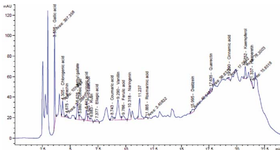
Figure 1. HPLC-phytochemical screening in Phoenix dactylifera rachis ethanolic extract
