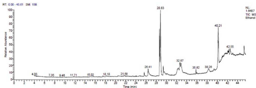
Figure 3. GC-MS phytochemical profiles of Phoenix dactylifera L. rachis ethanolic extract
