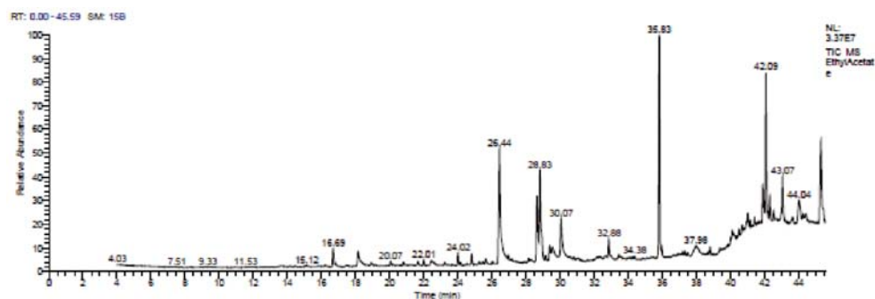
Figure 4. GC-MS phytochemical profiles of Phoenix dactylifera rachis ethyl acetate extract
