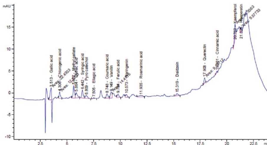
Figure 2. HPLC-phytochemical profiles in Phoenix dactylifera rachis ethyl acetate extract
