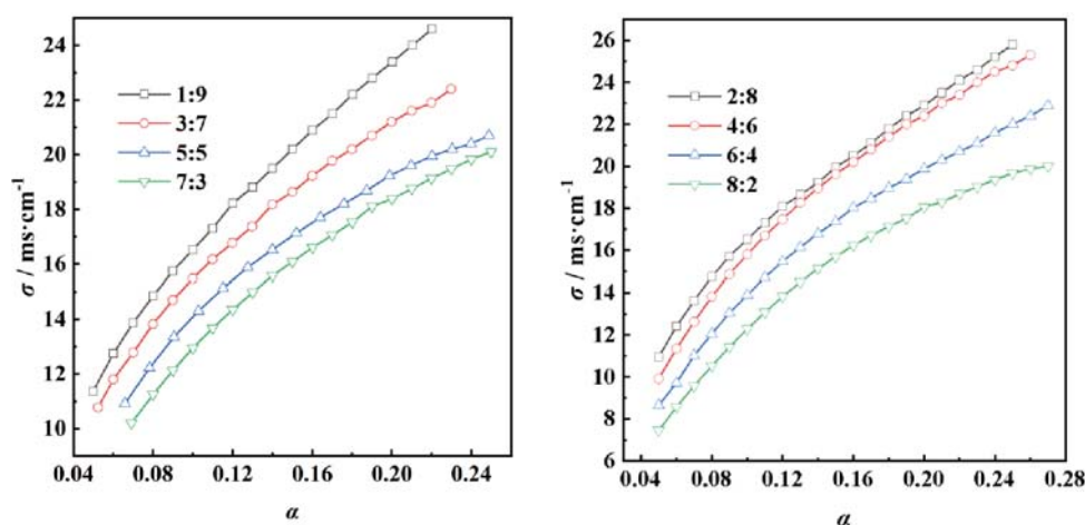
Figure 2. Variation of conductivity with concentration for different ratios of SLG/LHSB complex system
