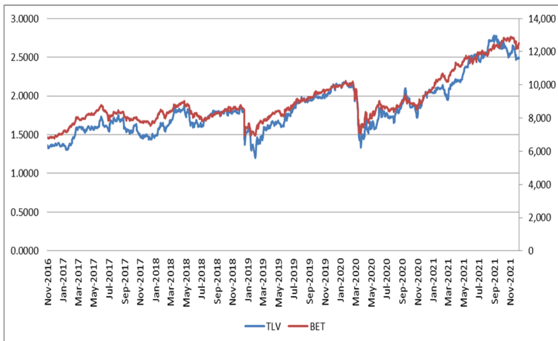
Figure 1. The evolution of TLV vs BET
