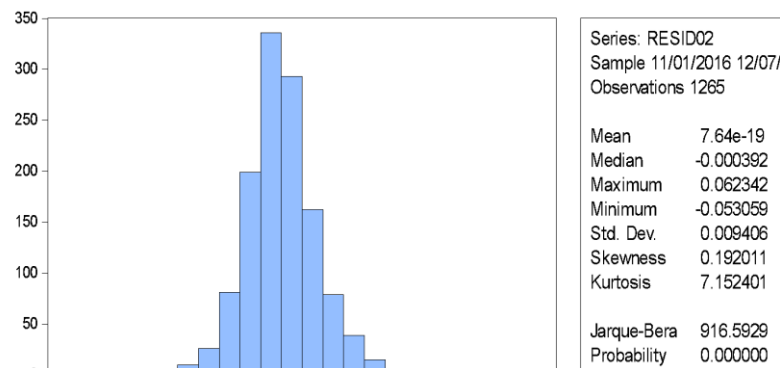
Figure 2. Descriptive statistics of the error term
