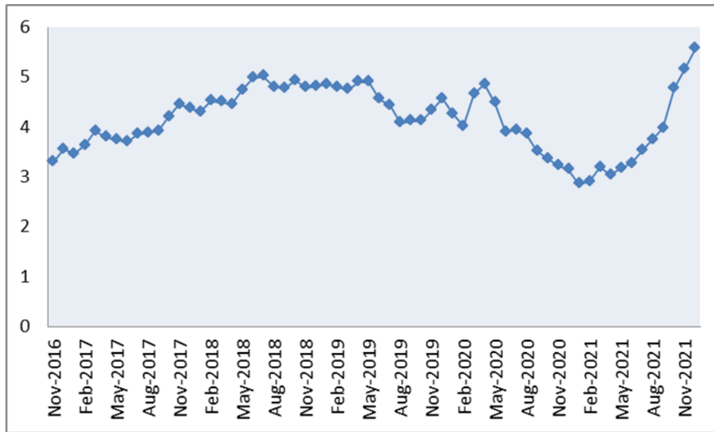
Figure 2. The evolution of the yield of 10-year government bonds (%)
