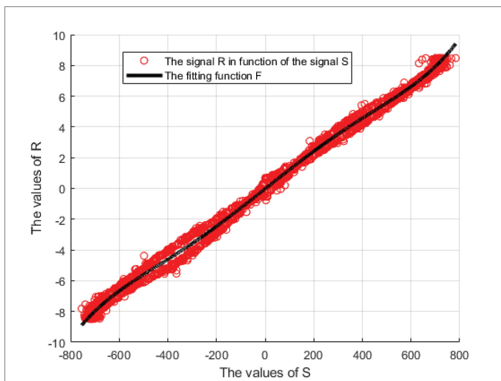
Figure 9. The scatter plot of R(S) and the estimated fitting function F .
