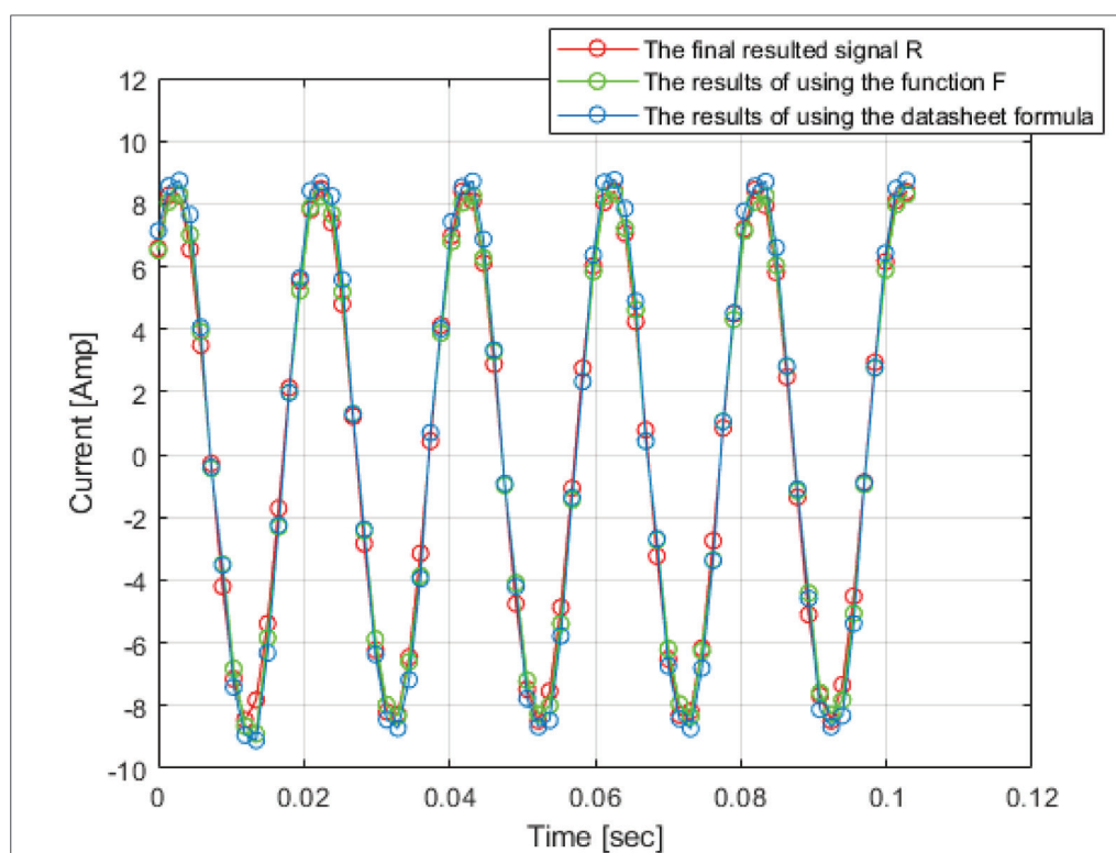
Figure 10. The results of applying F to S compared to the results of using the ACS712T datasheet formula and the estimated reference input R .
