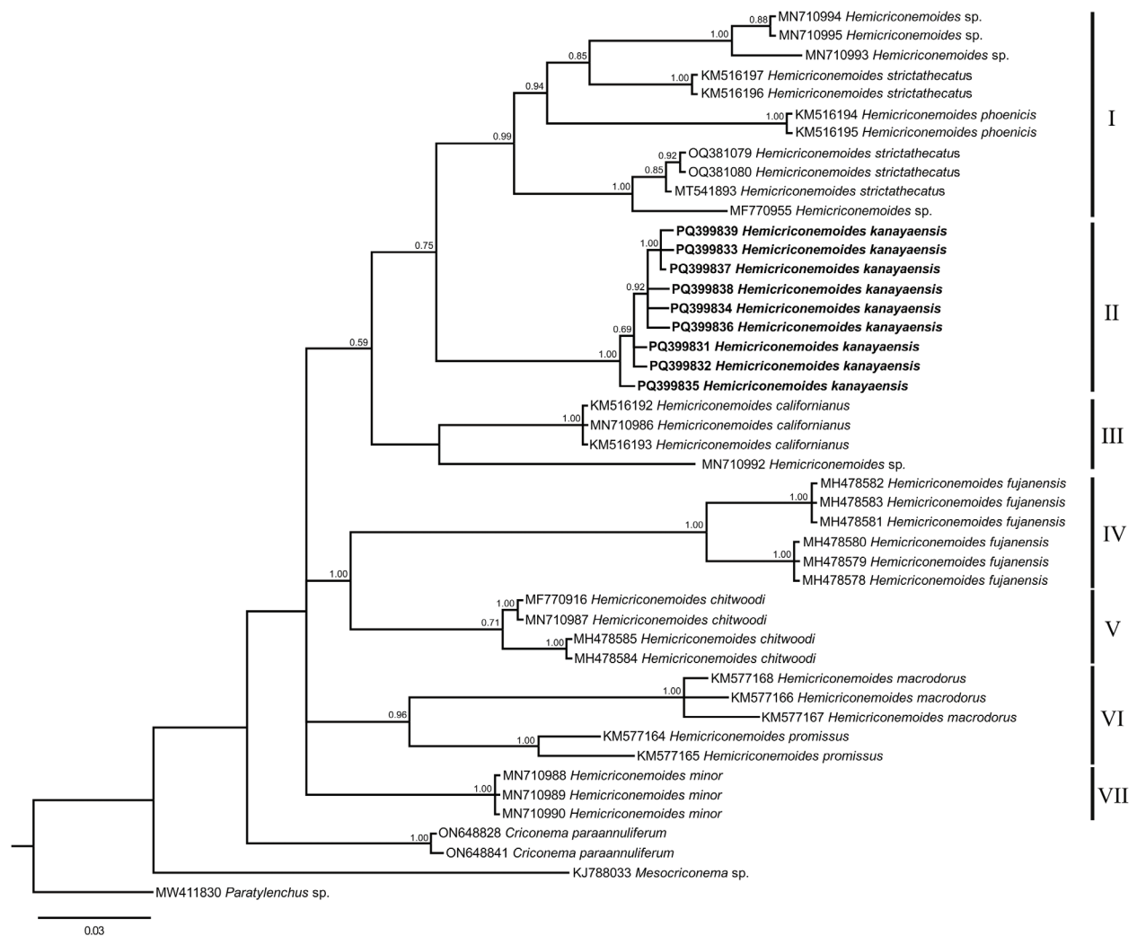
Figure 5: Phylogenetic tree based on Mitochondrial COI of Hemicriconemoides kanayaensis and Hemicriconemoides species. Bayesian 50% majority rule consensus tree as inferred from COI sequence alignment under General Time Reversible model across lineages along with a gamma distributed rates across sites (GTR+G). Posterior probabilities greater than 0.50 are given for appropriate clades. Newly obtained sequences in this study are shown in bold. Scale bar = expected changes per site.
