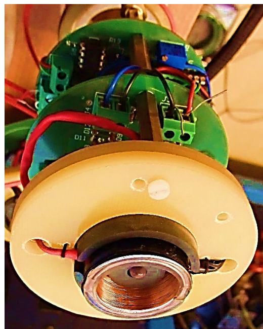
(b) Here, in the rotary part, is the secondary side of the transformer and a linear regulator stabilizing the output voltage at \pm 12 V.
