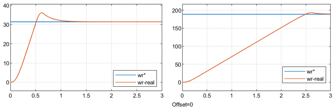
Figure 9. Rotor speed characteristics for f = 10\text{Hz} ; f = 60\text{Hz}
