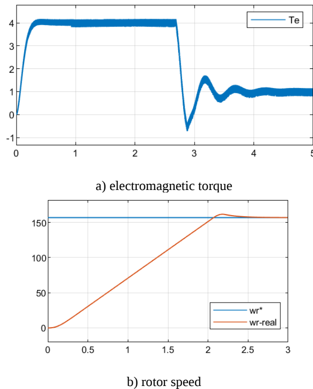
Figure 5. Mechanical characteristics of the asynchronous motor
