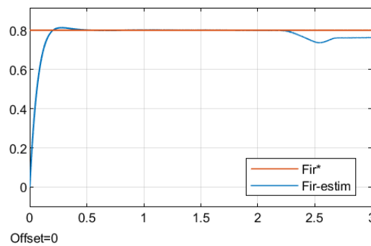
Figure 10. Rotor flux characteristics for f = 10\text{Hz} ; f = 60\text{Hz}
