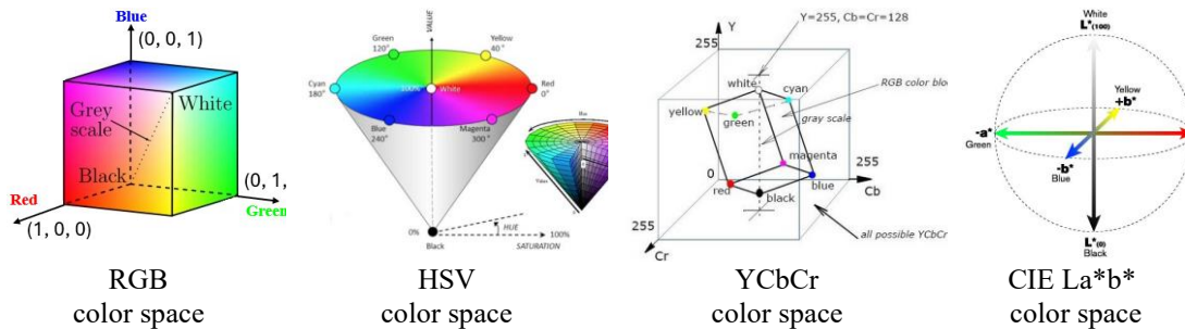
Figure 3. Colour spaces [26]
