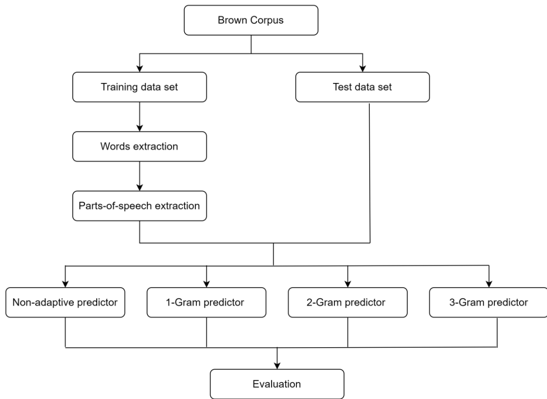
Figure 1. Application Architecture
