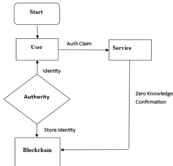
Figure 6. Working of self-sovereign identities (SSI)
