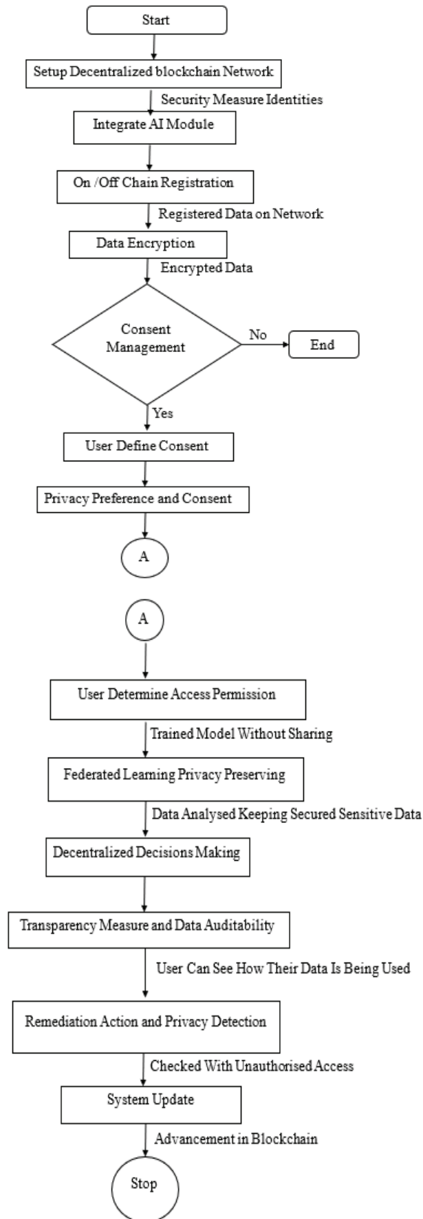
Figure 3. Flowchart that encompasses personal data protection and privacy control algorithm.
