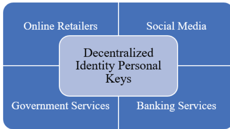
Figure 2. Decentralized Identity
