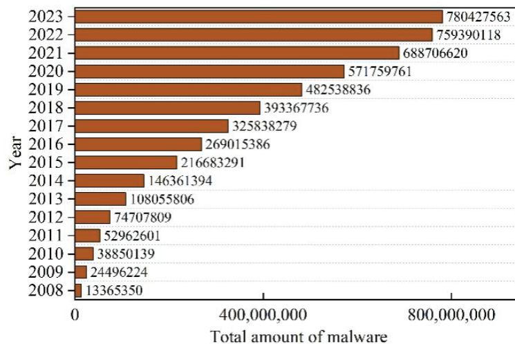
Figure 2. Total amount of malware per year [10]
