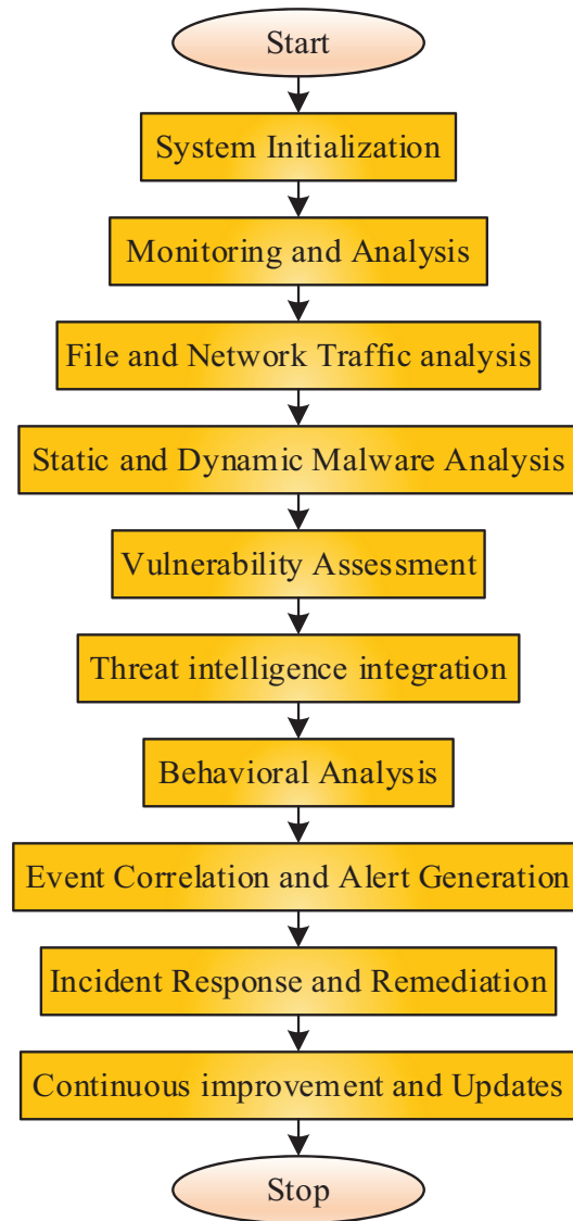
Figure 4. Flowchart that encompasses Malware Prevention and Detection (MP&D) algorithm
