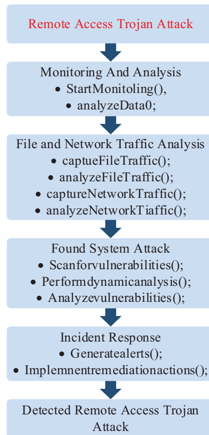
Figure 6. Action taken while Remote Action Trozen attack
