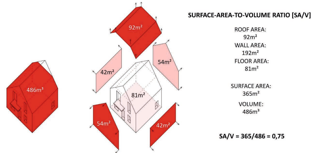
III. 5. Surface area to volume ratio of the house under study (by Mika P.)
