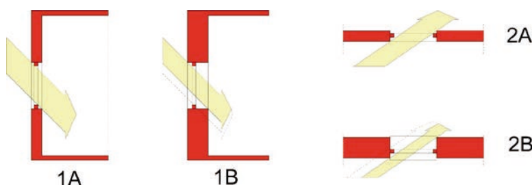
III. 11. Difference in interior insolation with a wall thickness of 26 cm (A) and 46.5 cm (B). Vertical sections (1) and plans (2). (by Mika P.)
