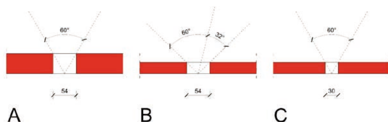
III. 12. The difference in the angle of manoeuvre and the width of the window aperture to meet the daylighting requirement with a wall thickness of 46.5 cm (A) and 26 cm (B and C), (by Mika P.).
