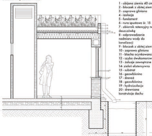
DETAL A | skala 1:20
