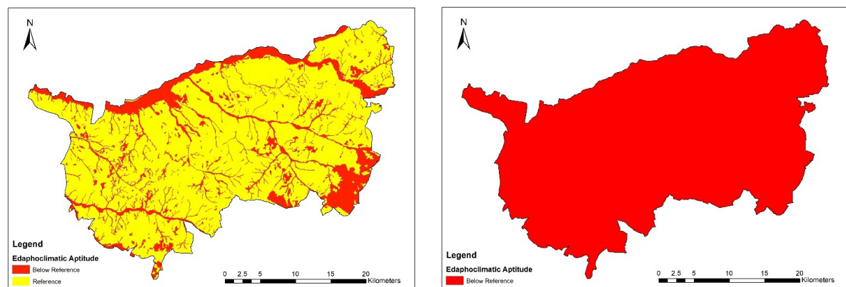
Fig. 2. Climatic aptitude for cork oak between: (a) 1994–2004; (b) 2000/05–2010/15 in the study area, Tagus Lezíria, Portugal.
