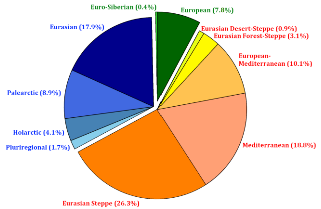
Fig. 4. Scheme of the geographical distribution of native plants in the Yelanetsky Steppe Nature Reserve flora: blue – widespread geoelements, red –geoelements of the "southern" geographical group, green –geoelements of the "northern" geographical group
