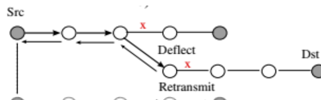
Fig. 1. Retransmission and deflection routing
