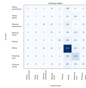
Proposed Model 3 (c)
