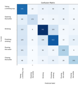
Proposed Model 8 (h)
