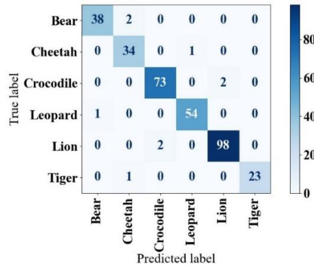
Fig. 10. Assessment of the proposed YOLOv8+EWC with the confusion matrix
