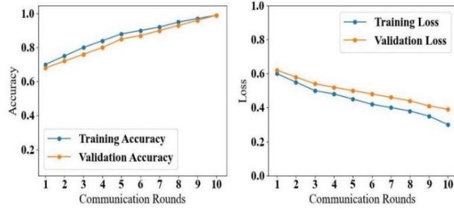
Fig. 12. Accuracy and loss curve of the FL unit
