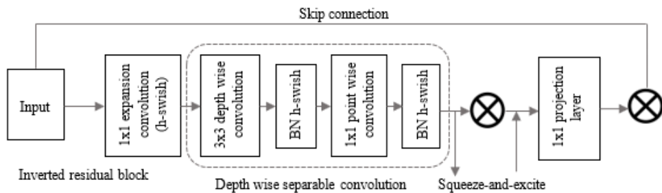
Fig. 4. Design of the MobileNetV3 architecture
