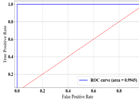
Fig. 13. Area under the Receiver Operating Characteristic Curve (AUC-ROC) of the FL unit
