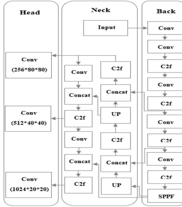
Fig. 3. Structure of the YOLOv8 architecture
