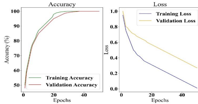
Fig. 9. Accuracy and loss curve of the proposed YOLOv8+EWC for 40 epochs
