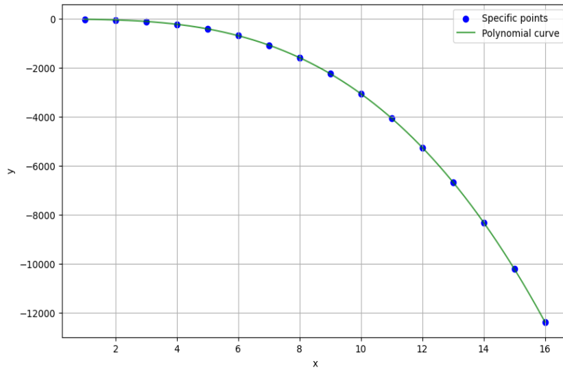
Fig. 2. Scatter plot for polynomial -3x^3 - 5x - 8
