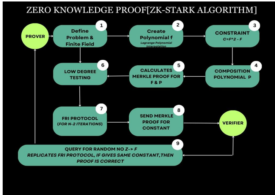
Fig. 1. ZK-STARK detail stepwise algorithm
