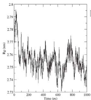
Radius of gyration (total and around axes)
