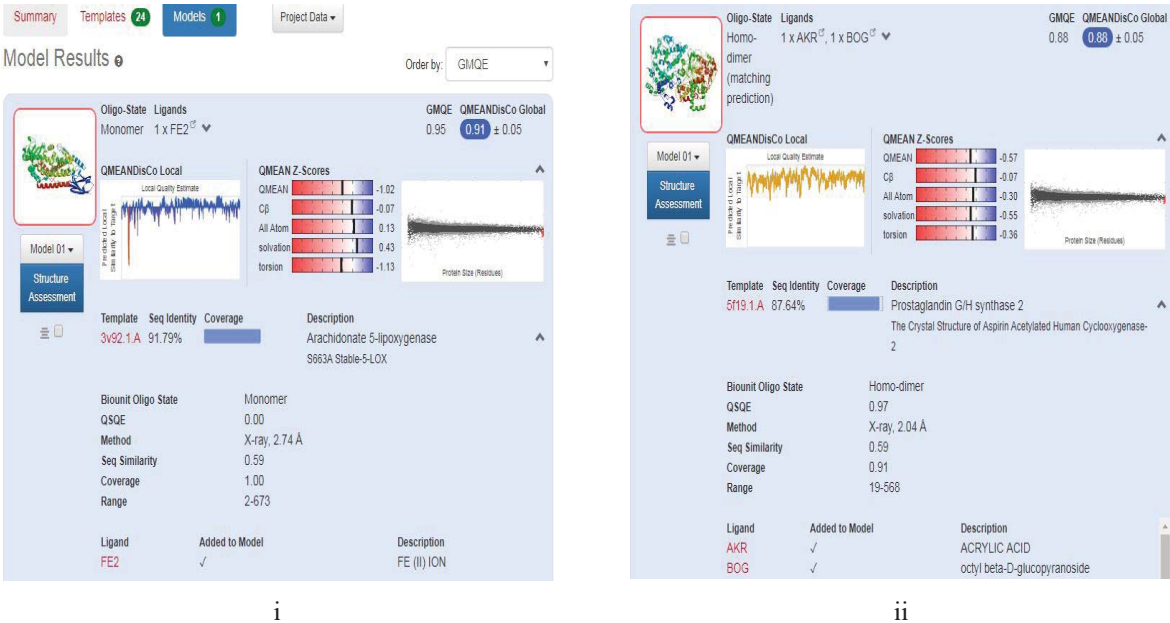
Fig. 1. The 3D Swiss model crystal structures of COX and LOX
