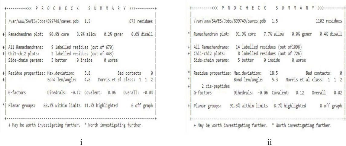
Fig. 2. The PROCHECK summary of 3D Swiss model COX and LOX crystal structures
