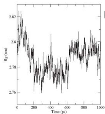
Radius of gyration (total and around axes)
