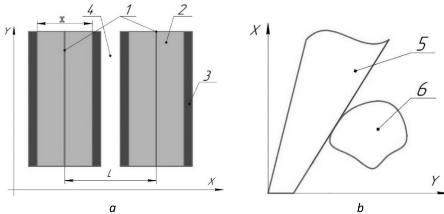
Figure 2. Zones of influence of harrow teeth on the soil during operation: a – horizontal plane; b – vertical plane; ( L ) – distance between teeth in the direction of machine movement; 1 – traces of adjacent harrow teeth; 2 – strips in the zone where soil loosening occurs under the influence of harrow teeth; 3 – zones where the influence of the working bodies is insufficient for soil loosening; 4 – zone where the teeth do not affect soil aggregates at all; 5 – tooth; 6 – soil aggregate (clod).
