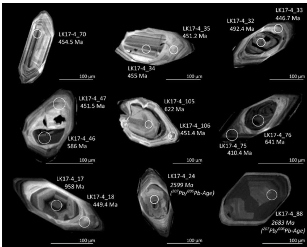
Figure 6: Cathodoluminescence images of exemplary zircons of LK17-4. White circles are laser ablation spots marked with measured \text{U}^{238}/\text{Pb}^{206} -ages unless otherwise marked.
