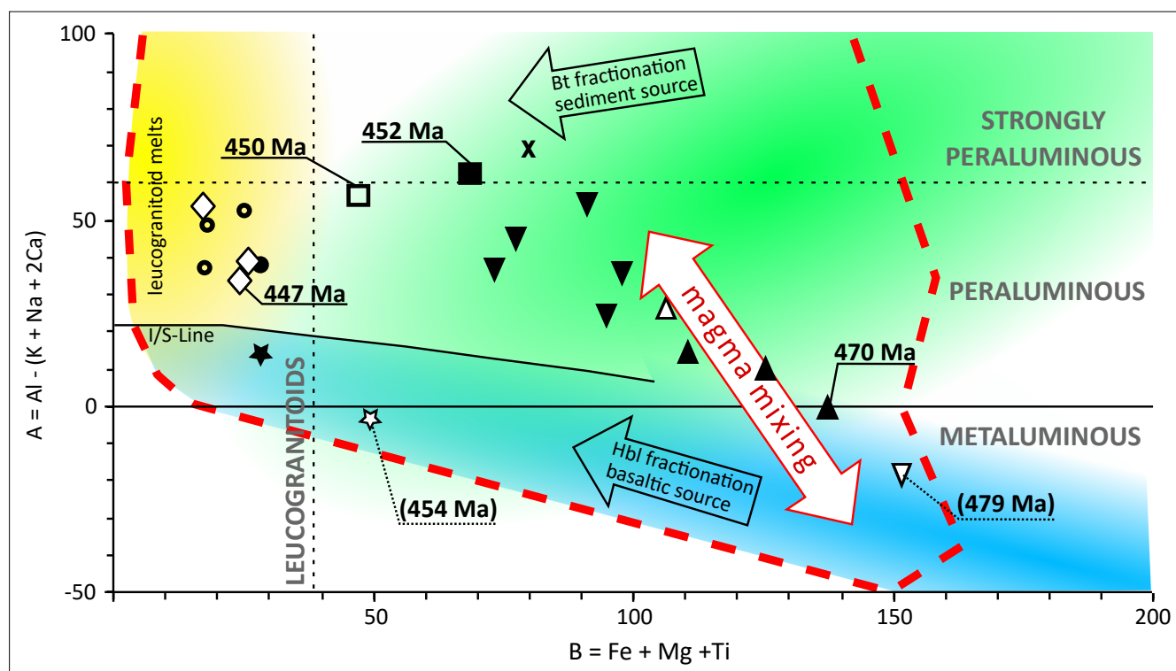
Figure 10: Discrimination diagram after Debon and Le Fort (1988) and Zurbriegen (2015, 2020) with data from orthogneisses of this study, Bargossi et al. (2010) and Schindlmayr (1999). Ages for the samples TX38, TX44, LK17-3 and LK17-4 are from this study. Ages in brackets are from Klötzli et al. (2008) (454 Ma) and Siegesmund et al. (2021) (479 Ma). Colored fields are leucogranitoid melts (yellow), sediments (green), high-temperature I-type granitoids (blue) and low-temperature I- and S-types (red line). The I/S-line is used after Villaseca et al. (1998). Symbols as in Figure 9.
