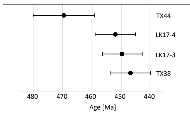
Figure 11: Time scale of magmatic growth concordia ages of samples TX38, TX44, LK17-3 and LK17-4 with 2σ uncertainty-bars.
