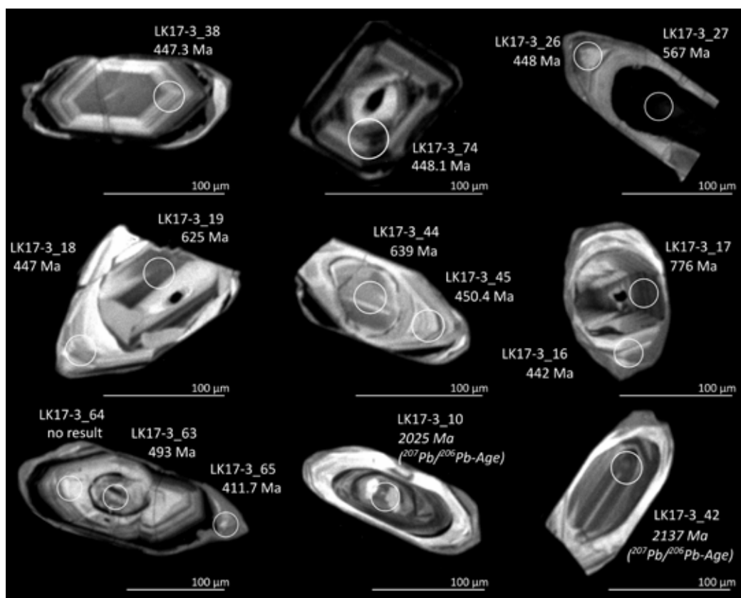
Figure 5: Cathodoluminescence images of exemplary zircons of LK17-3. White circles are laser ablation spots marked with measured \text{U}^{238}/\text{Pb}^{206} -ages unless otherwise marked.
