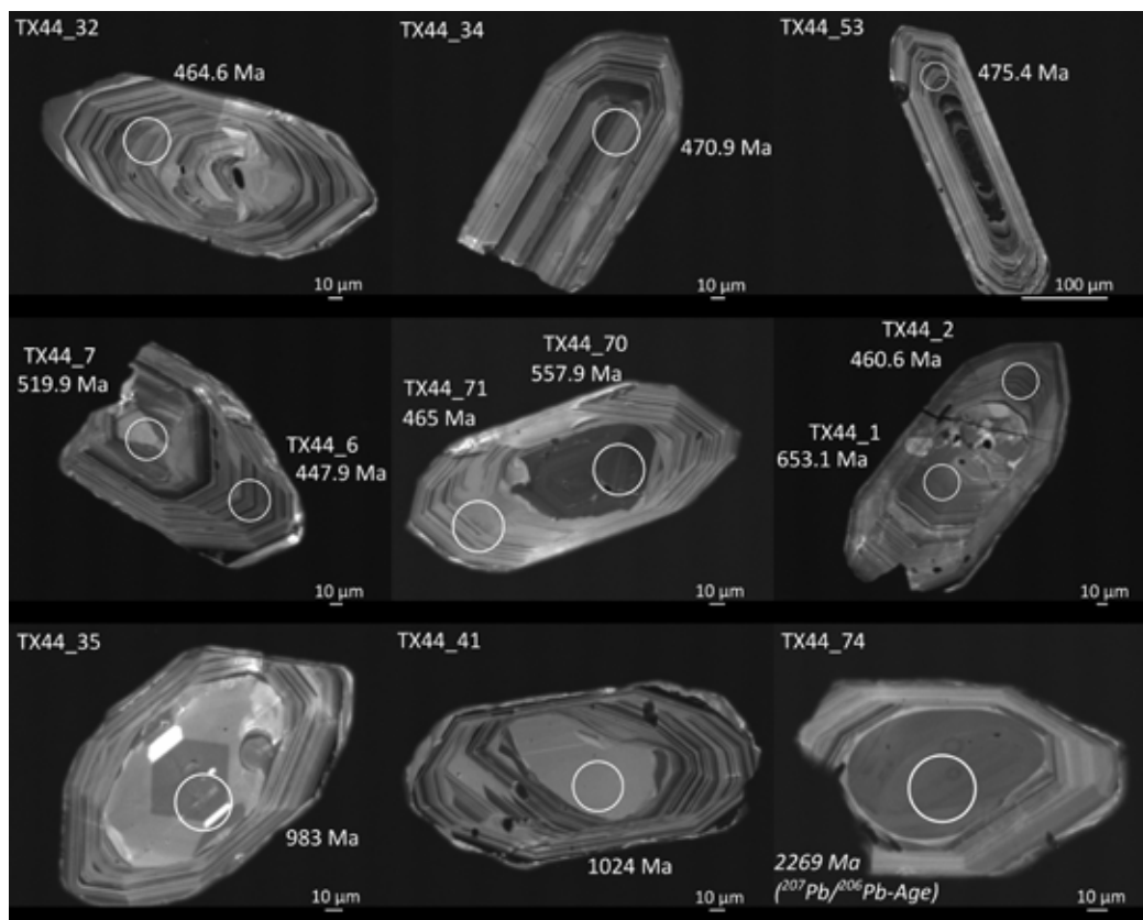
Figure 4: Cathodoluminescence images of exemplary zircons of TX44. White circles are laser ablation spots marked with measured U^{238}/Pb^{206} -ages unless otherwise marked.
