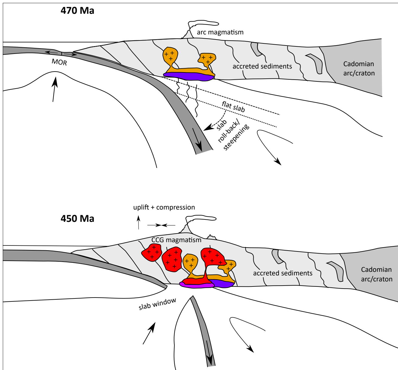
Figure 12: Tectonic model of the Ordovician magmatism in the Texel complex for the time steps 470 Ma and 450 Ma, with underplating basaltic melts (purple and pink) and emplaced granitoids (orange and red), respectively. The observed differentiation trend is linked to slab steepening/roll-back and mid ocean ridge subduction. See text for details.
