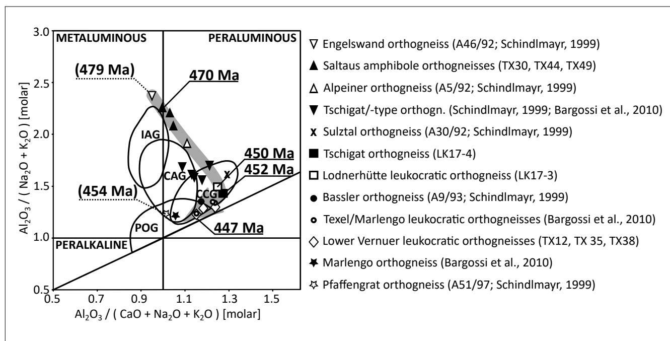
Figure 9: Discrimination diagram of granitoids after Maniar and Piccoli (1989) with geochemical data from orthogneisses of this study, Bargossi et al. (2010) and Schindlmayr (1999). Ages for the samples TX38, TX44, LK17-3 and LK17-4 are from this study. Ages in brackets are from Klötzli et al. (2008) (454 Ma) and Siegesmund et al. (2021) (479 Ma). The arrow marks the temporal differentiation trend.
