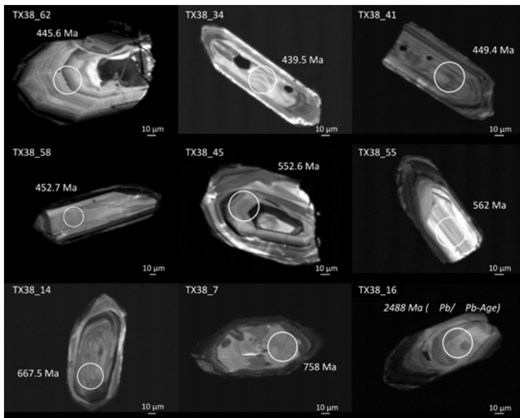
Figure 3: Cathodoluminescence images of exemplary zircons of TX38. White circles are laser ablation spots marked with measured U^{238}/Pb^{206} -ages unless otherwise marked.
