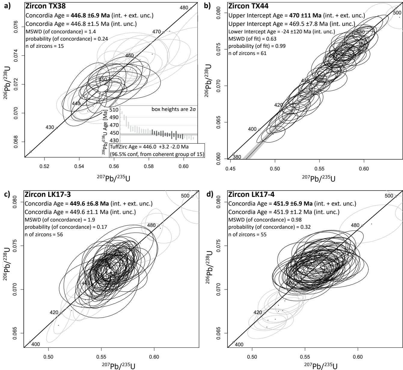
Figure 7: Concordia ages for last magmatic growth in samples (a) TX38, (b) TX44, (c) LK17-3, (d) LK17-4.
