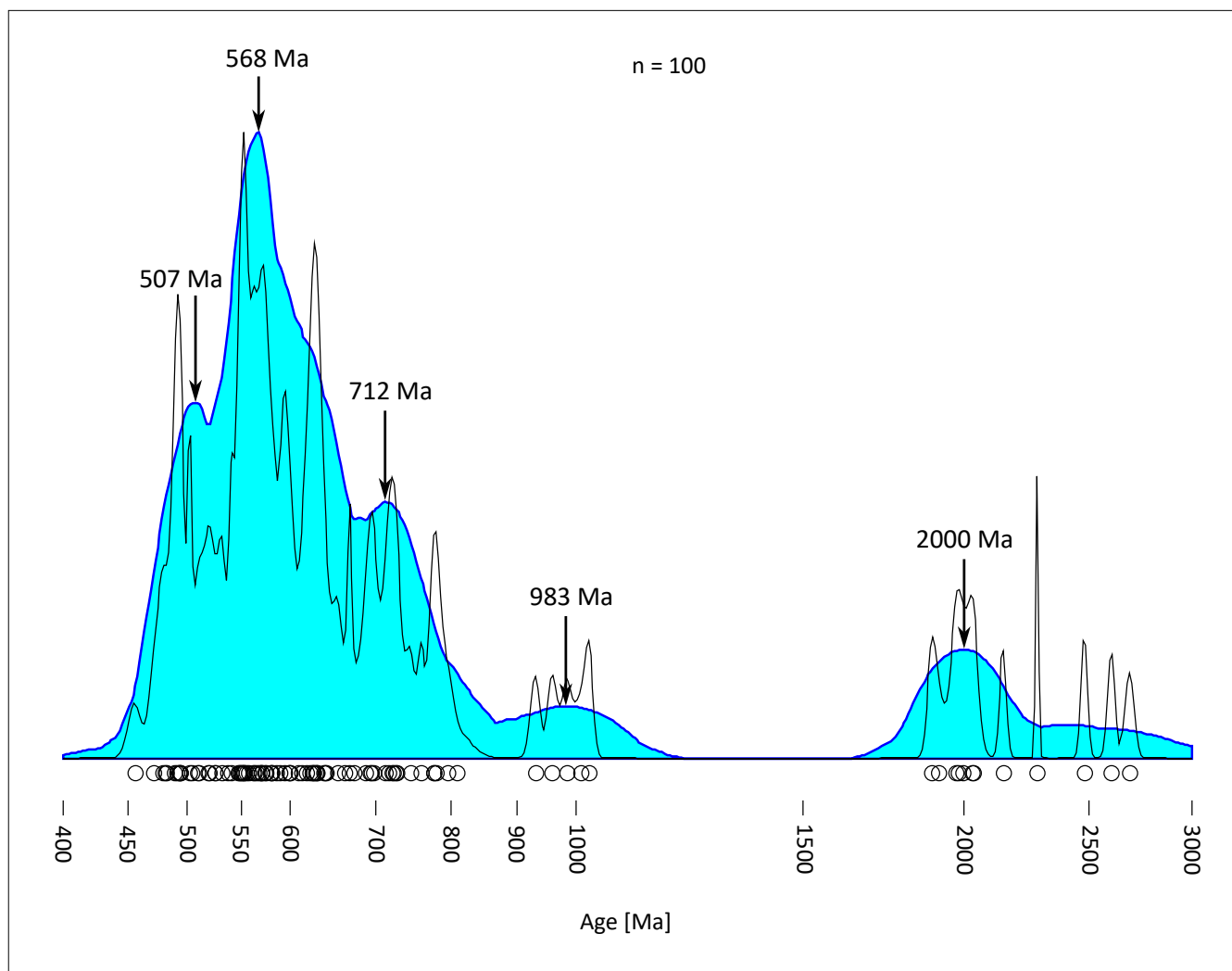
Figure 8: Inherited zircon cores combined from samples TX38, TX44, LK17-3 and LK17-4 in a Kernel Density Estimation (blue) and a probability density plot (black). Cores younger than 1500 Ma are plotted with U^{238}/Pb^{206} -ages, cores older than 1500 Ma with Pb^{207}/Pb^{206} -ages.
