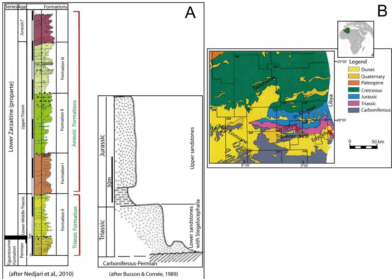
Fig. 1. A – Stratigraphical log of the Triassic series (Zarzaitine Formation) following previous studies. The red intervals refer to ages assigned by Ait Ouali et al. (2011); B – Location and geological map of the study area (Beicip-Sonatrach, 1975). Stars indicate study sites. 1: coordinates: 27°48'33.76" N - 9°21'10.13" E; 2: coordinates: 27°43'51.3" N - 9°52'2056" E.
